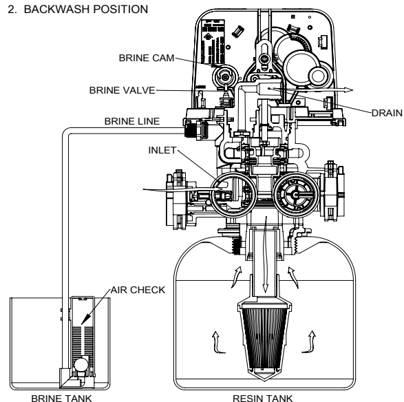
2. BACKWASH POSITION
